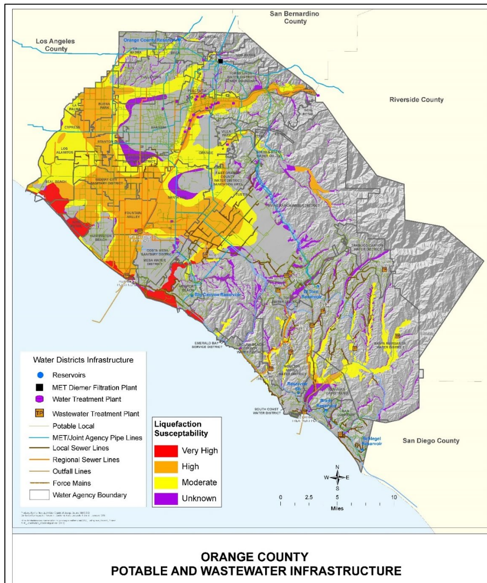
Exhibit 3-20. Liquefaction Susceptibility Zones
